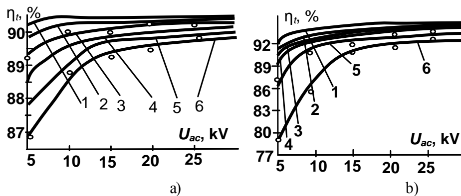
Fig. 3. Dependences of energetic efficiency of HVGD electrodes' system on acceleration voltage, voltage of additional discharge (a) and operation pressure (b):
