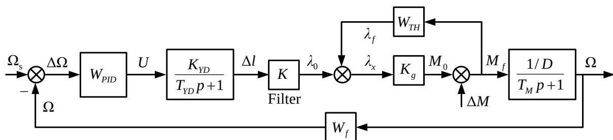
Fig. 1. Structural diagram, which reflects the characteristic of the work of the GDGU
