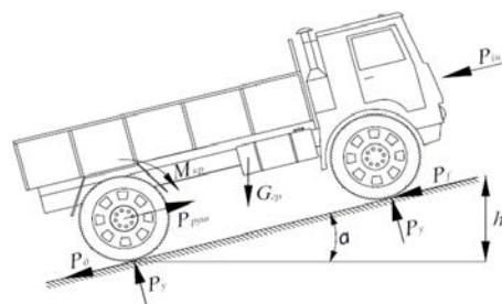
Fig. 6. Power load of a military vehicle
